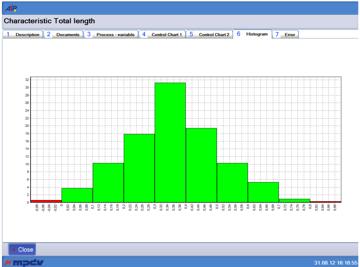
Figure: Index tab "Histogram" in the information on characteristics
