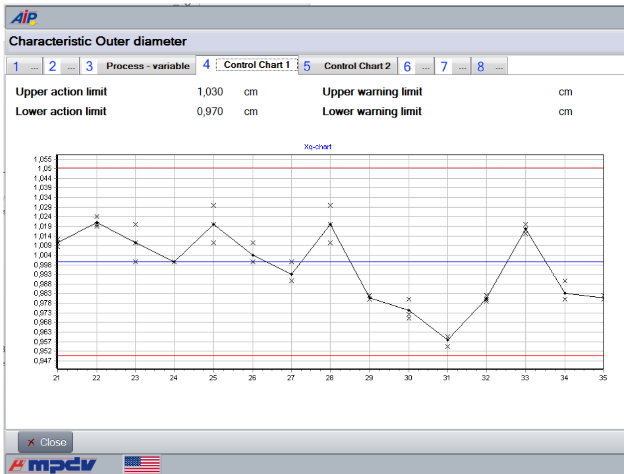
Figure: Index tab "Control chart #1" in information on characteristics
